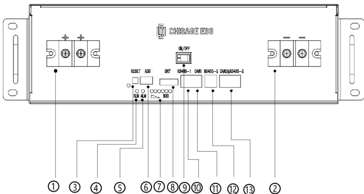
Fig. 3-5 MOON5-R PACK interface
