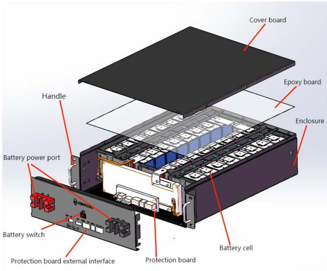
Fig. 3-1 MOON5-R PACK mechanical structure 1
