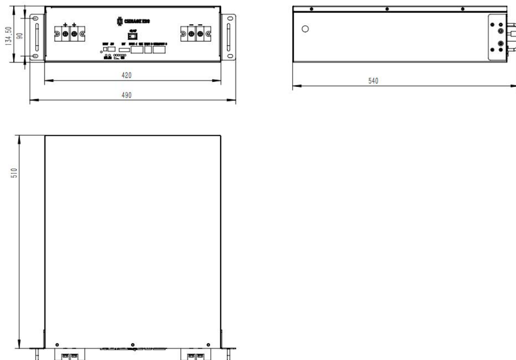
Fig. 3-3 MOON5-R PACK dimension drawing
