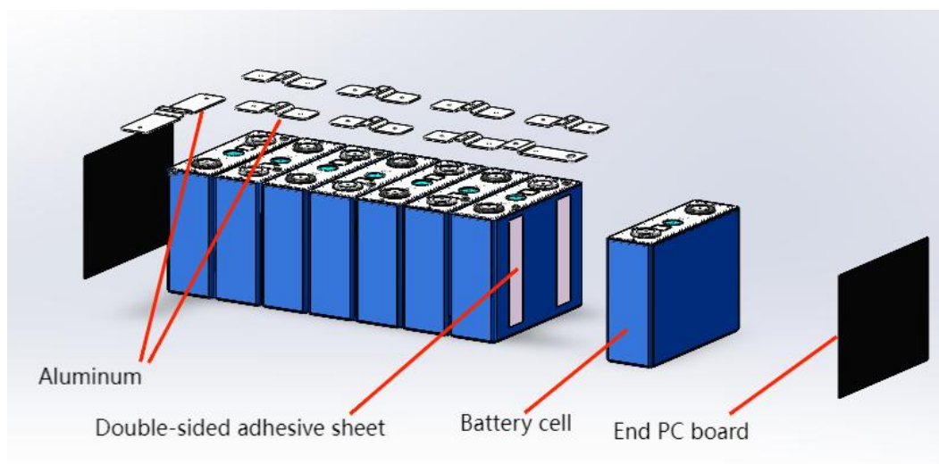
Fig. 3-2 MOON5-R PACK mechanical structure 2
