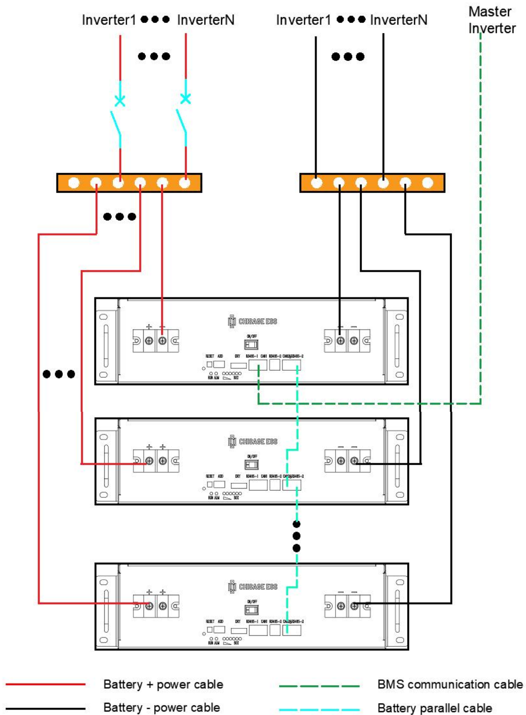
Fig. 4-2 Multi MOON5-R PACK + multi inverter diagram
