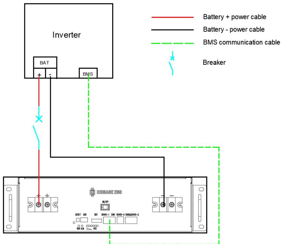
Fig. 4-1 Single MOON5-R PACK + single inverter diagram
